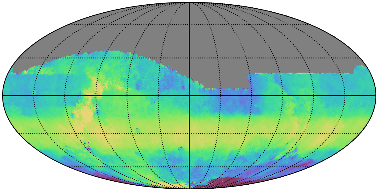
too_elab_r8_d3_ugrizy_v3.4_10yrs All sky z band: Median HA
