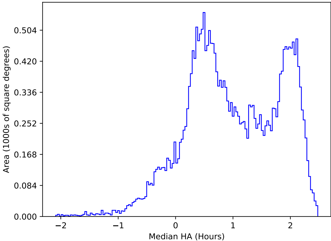
too_elab_r8_d3_ugrizy_v3.4_10yrs All sky z band: Median HA
