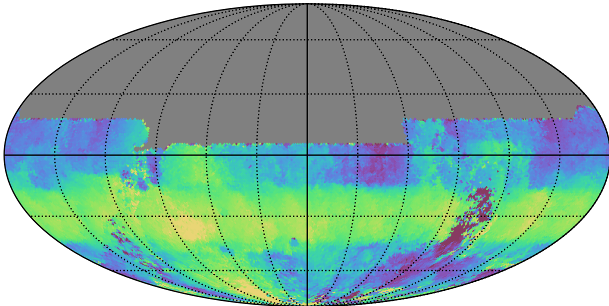
too_elab_r8_d3_ugrizy_v3.4_10yrs All sky u band: Median HA
