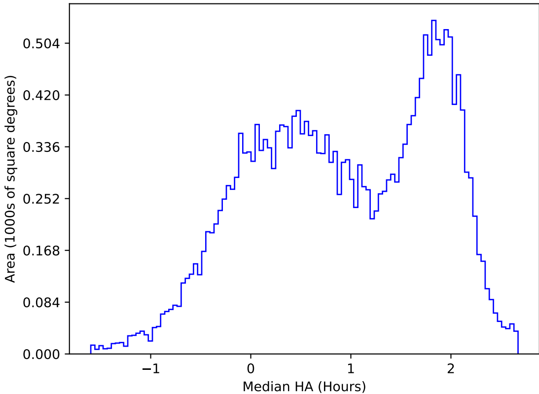
too_elab_r8_d3_ugrizy_v3.4_10yrs All sky u band: Median HA
