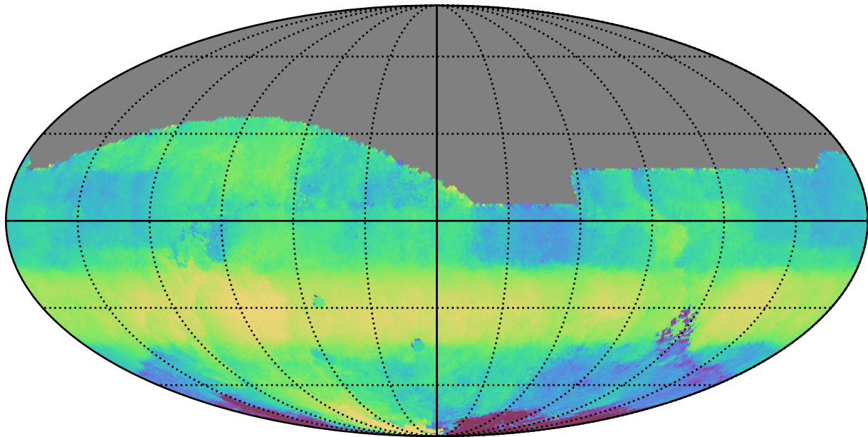
too_elab_r8_d3_ugrizy_v3.4_10yrs All sky r band: Median HA
