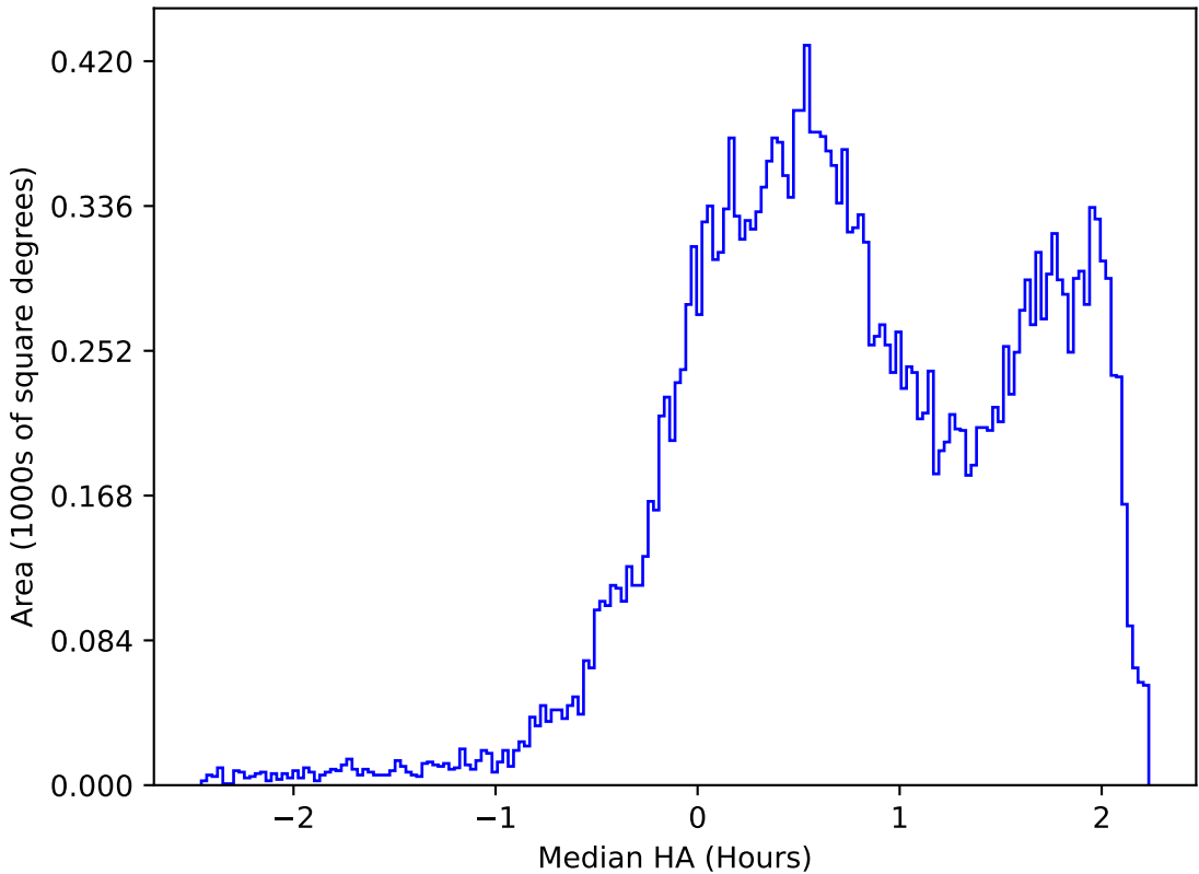
too_elab_r8_d3_ugrizy_v3.4_10yrs All sky r band: Median HA
