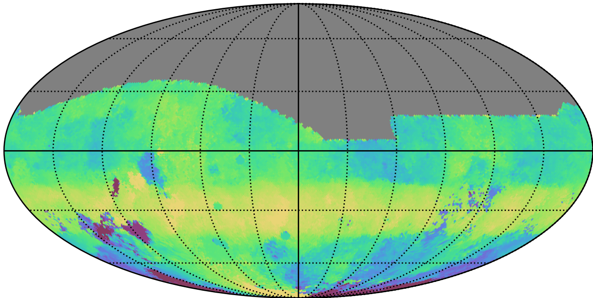
too_elab_r8_d3_ugrizy_v3.4_10yrs All sky g band: Median HA
