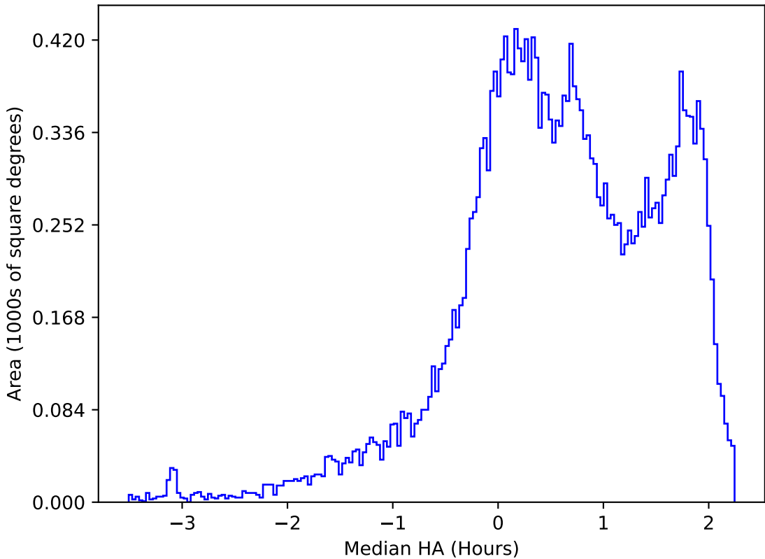
too_elab_r8_d3_ugrizy_v3.4_10yrs All sky g band: Median HA
