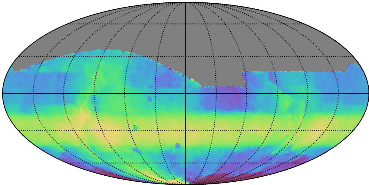
too_elab_r8_d3_ugrizy_v3.4_10yrs All sky all bands: Median HA
