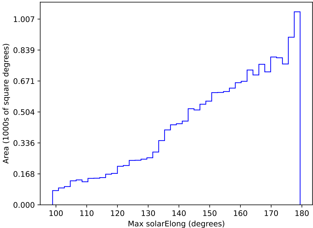
too_elab_r8_d3_ugrizy_v3.4_10yrs WFD z band: Max solarElong
