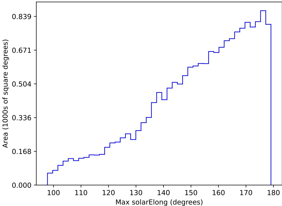
too_elab_r8_d3_ugrizy_v3.4_10yrs WFD u band: Max solarElong
