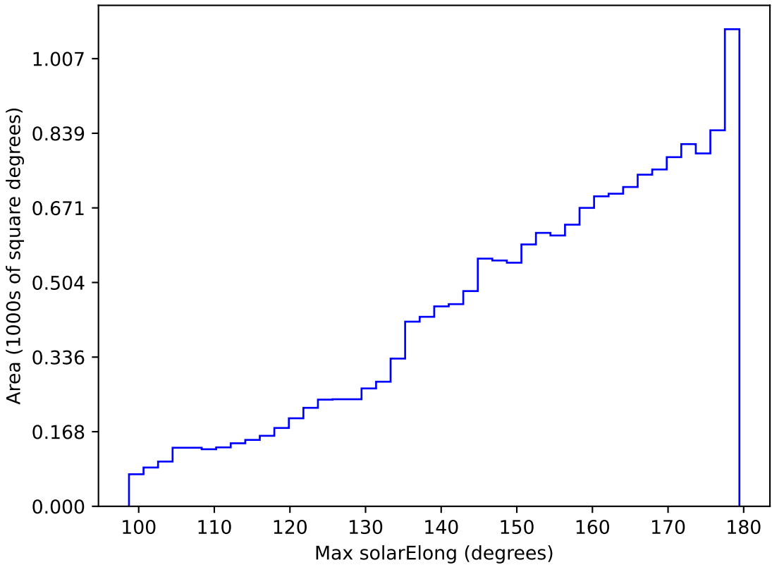
too_elab_r8_d3_ugrizy_v3.4_10yrs WFD r band: Max solarElong
