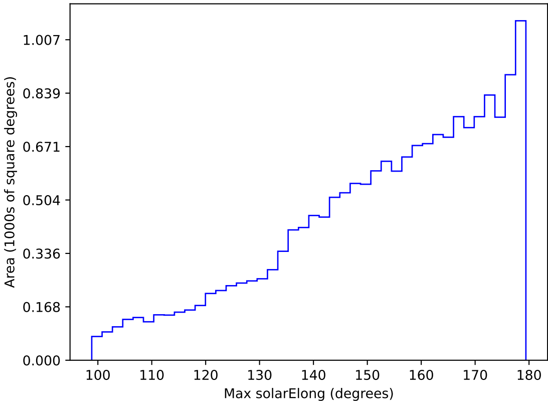
too_elab_r8_d3_ugrizy_v3.4_10yrs WFD i band: Max solarElong
