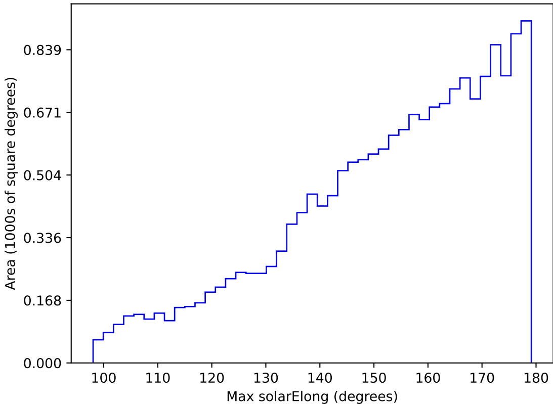
too_elab_r8_d3_ugrizy_v3.4_10yrs WFD g band: Max solarElong
