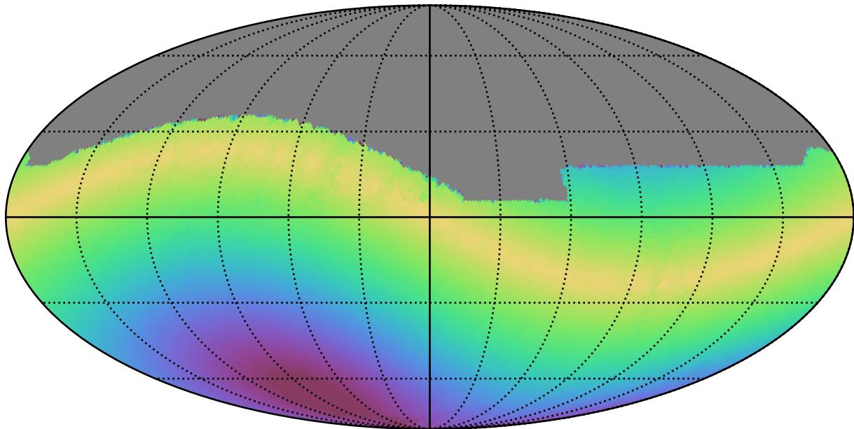
too_elab_r8_d3_ugrizy_v3.4_10yrs All sky z band: Max solarElong
