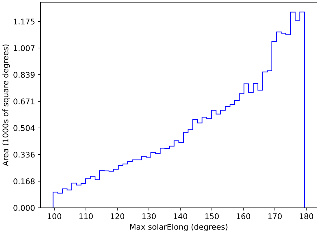
too_elab_r8_d3_ugrizy_v3.4_10yrs All sky z band: Max solarElong
