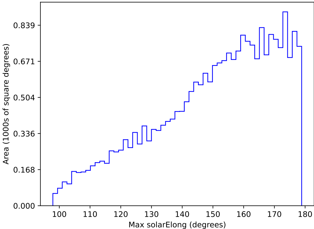
too_elab_r8_d3_ugrizy_v3.4_10yrs All sky u band: Max solarElong
