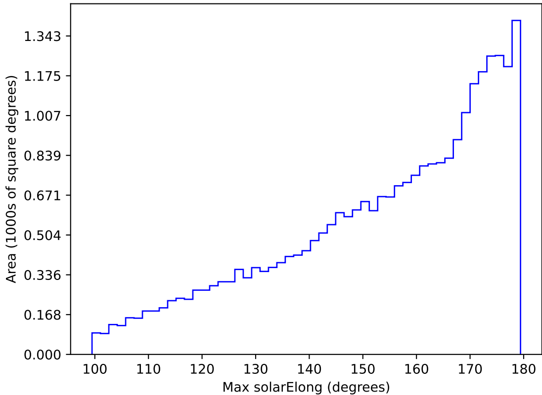
too_elab_r8_d3_ugrizy_v3.4_10yrs All sky r band: Max solarElong
