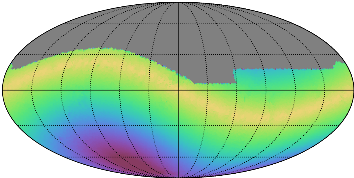
too_elab_r8_d3_ugrizy_v3.4_10yrs All sky g band: Max solarElong
