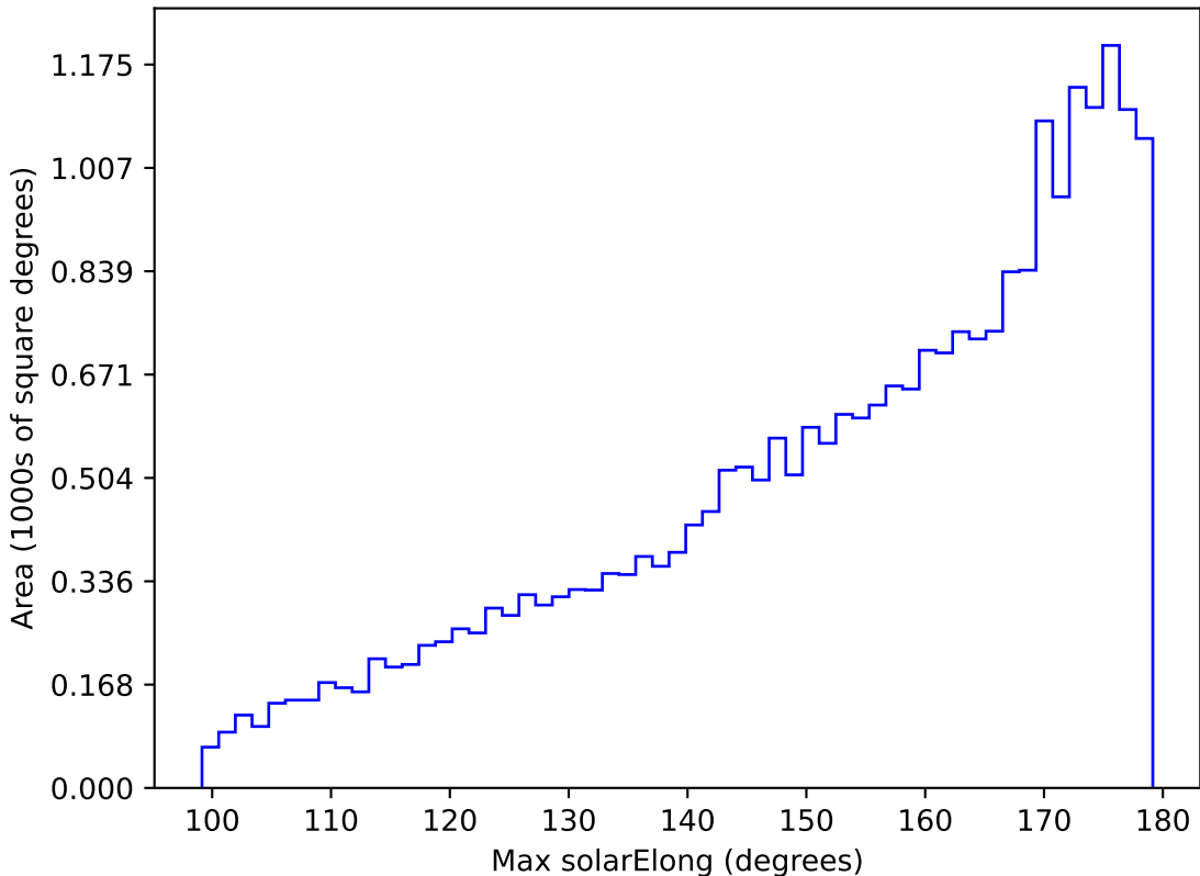
too_elab_r8_d3_ugrizy_v3.4_10yrs All sky g band: Max solarElong
