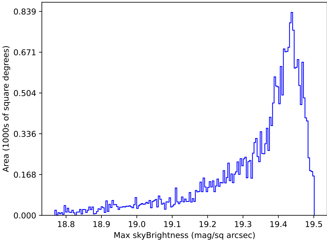
too_elab_r8_d3_ugrizy_v3.4_10yrs Yr 1 z band: Max skyBrightness
