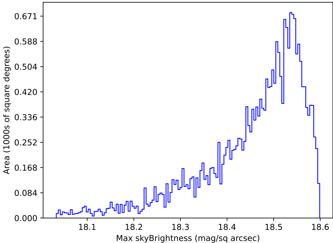
too_elab_r8_d3_ugrizy_v3.4_10yrs Yr 1 y band: Max skyBrightness
