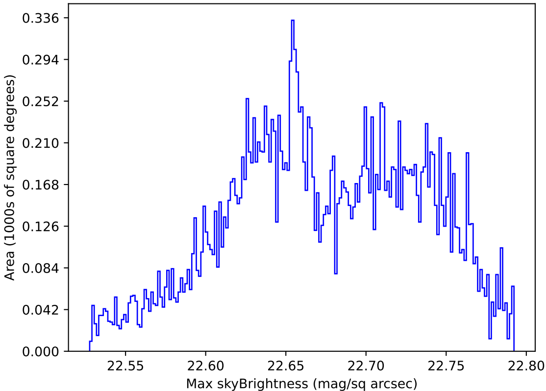
too_elab_r8_d3_ugrizy_v3.4_10yrs Yr 1 u band: Max skyBrightness
