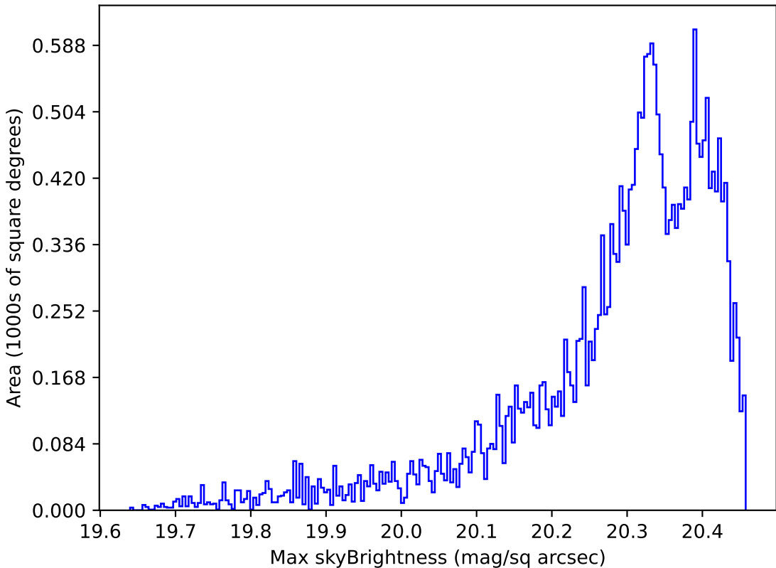
too_elab_r8_d3_ugrizy_v3.4_10yrs Yr 1 i band: Max skyBrightness
