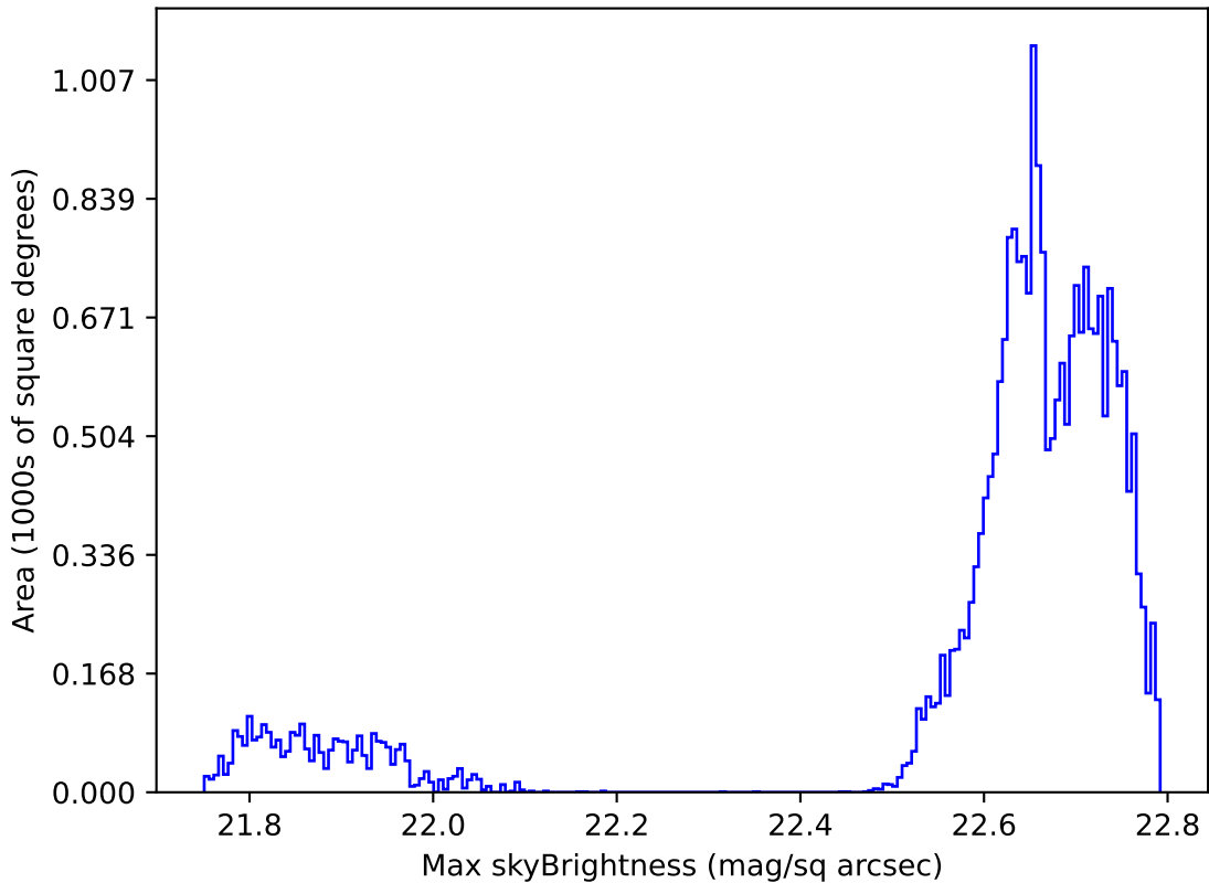
too_elab_r8_d3_ugrizy_v3.4_10yrs Yr 1 all bands: Max skyBrightness
