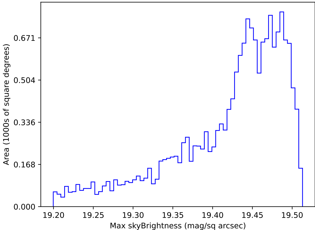
too_elab_r8_d3_ugrizy_v3.4_10yrs WFD z band: Max skyBrightness
