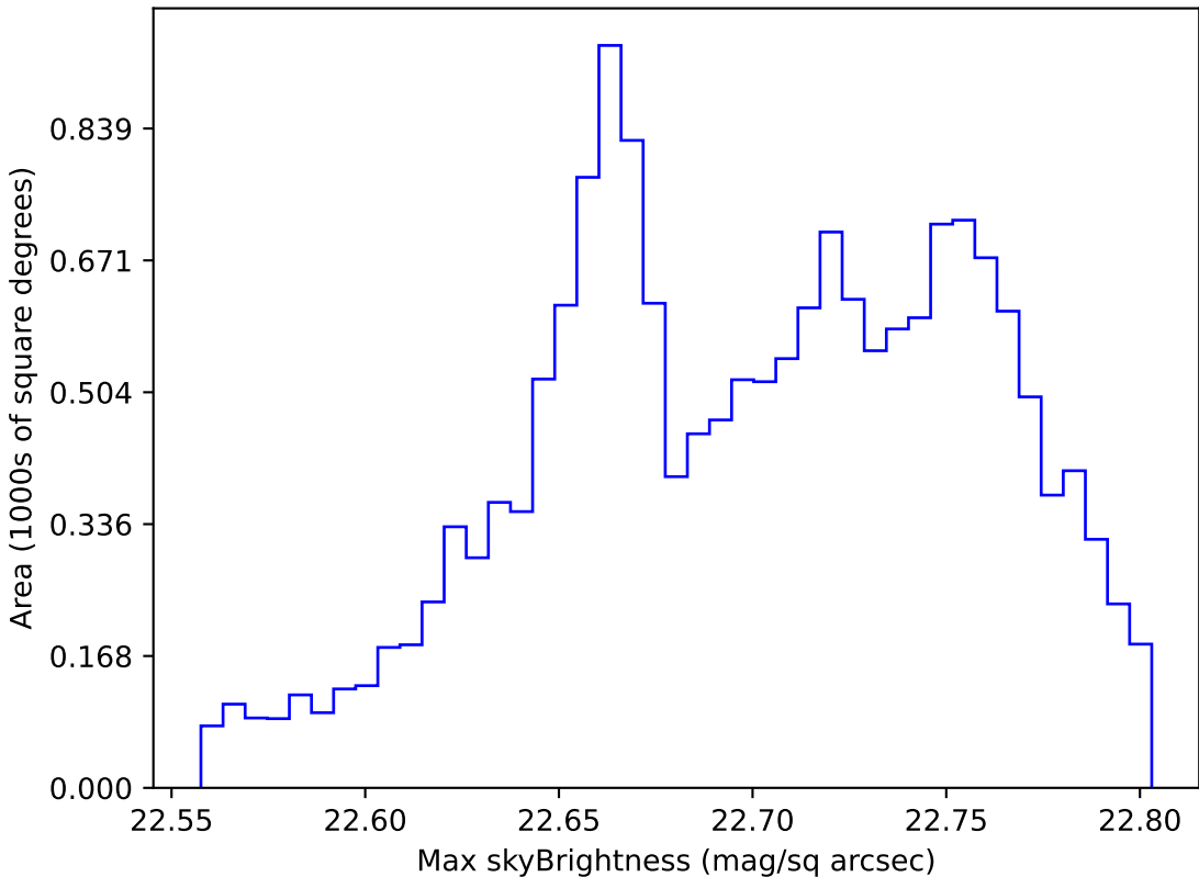
too_elab_r8_d3_ugrizy_v3.4_10yrs WFD u band: Max skyBrightness
