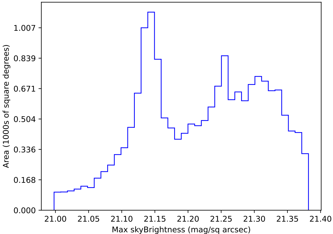
too_elab_r8_d3_ugrizy_v3.4_10yrs WFD r band: Max skyBrightness
