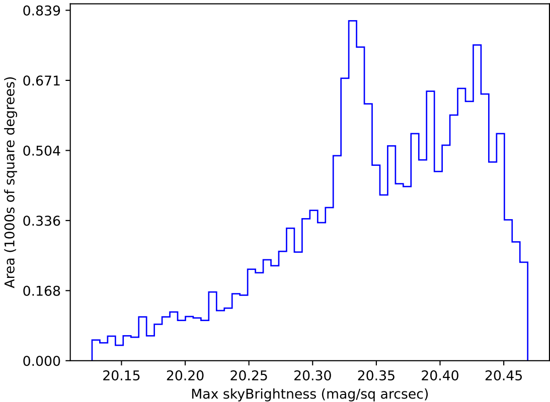
too_elab_r8_d3_ugrizy_v3.4_10yrs WFD i band: Max skyBrightness
