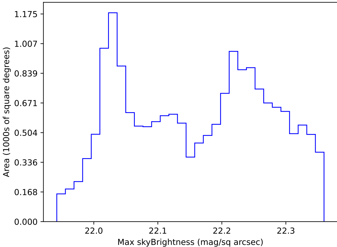
too_elab_r8_d3_ugrizy_v3.4_10yrs WFD g band: Max skyBrightness
