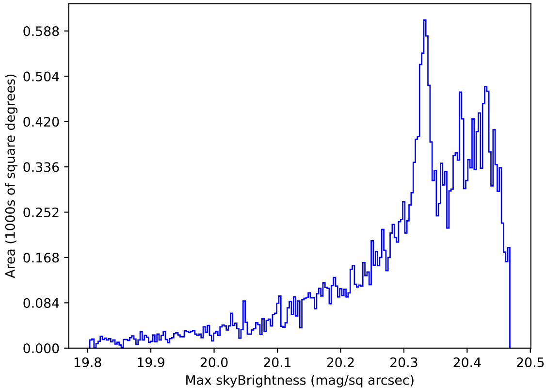
too_elab_r8_d3_ugrizy_v3.4_10yrs All sky i band: Max skyBrightness
