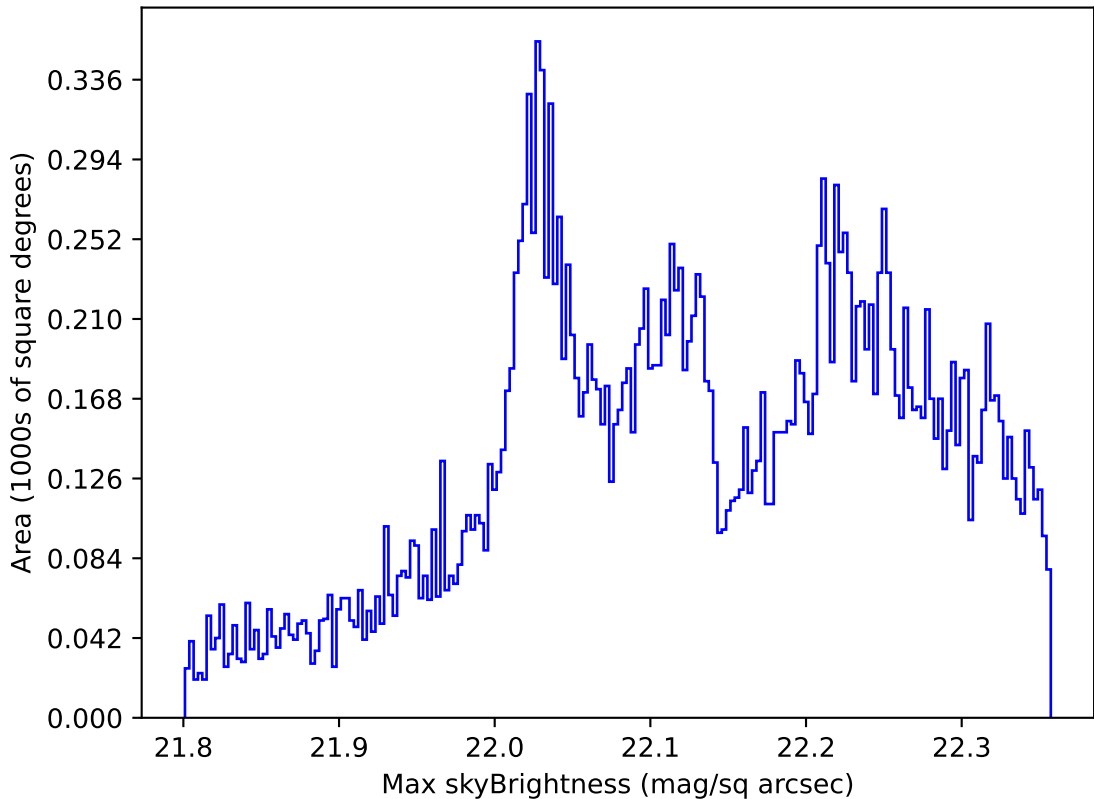
too_elab_r8_d3_ugrizy_v3.4_10yrs All sky g band: Max skyBrightness
