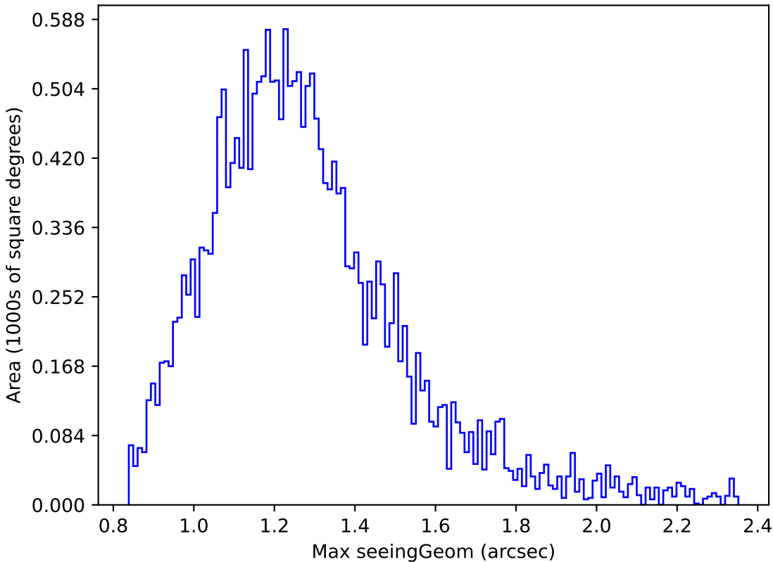
too_elab_r8_d3_ugrizy_v3.4_10yrs Yr 1 y band: Max seeingGeom
