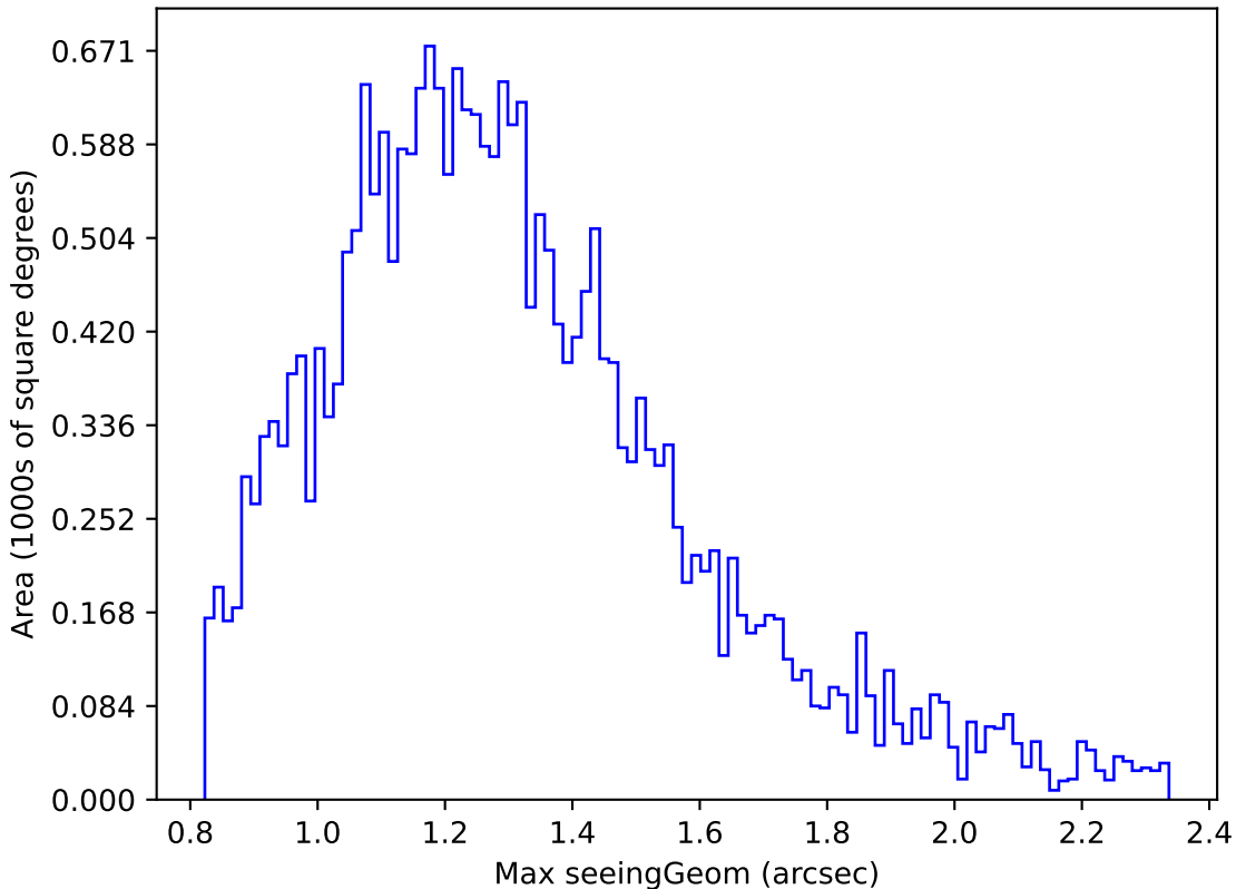
too_elab_r8_d3_ugrizy_v3.4_10yrs Yr 1 i band: Max seeingGeom
