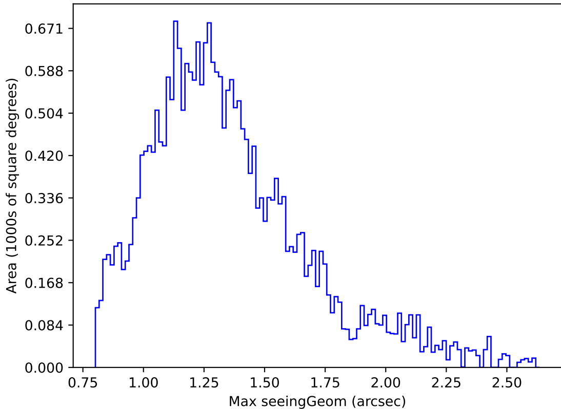
too_elab_r8_d3_ugrizy_v3.4_10yrs Yr 1 g band: Max seeingGeom
