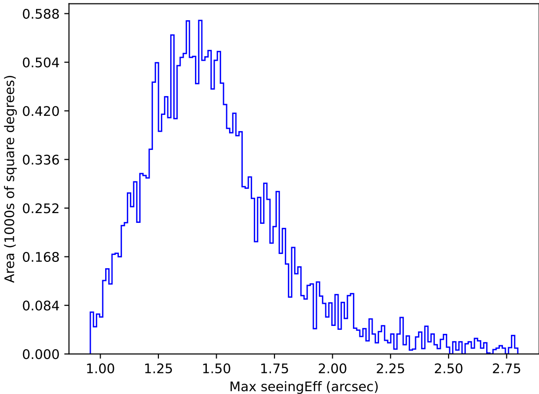
too_elab_r8_d3_ugrizy_v3.4_10yrs Yr 1 y band: Max seeingEff
