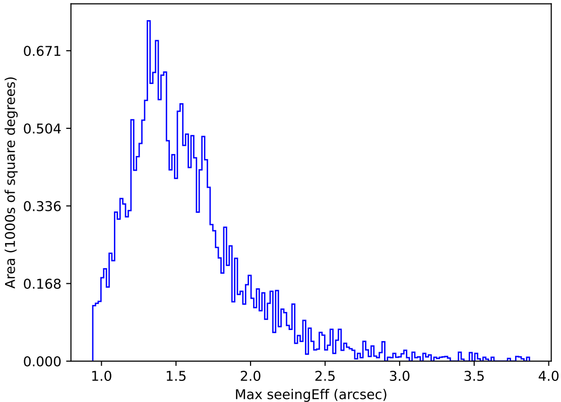
too_elab_r8_d3_ugrizy_v3.4_10yrs Yr 1 u band: Max seeingEff
