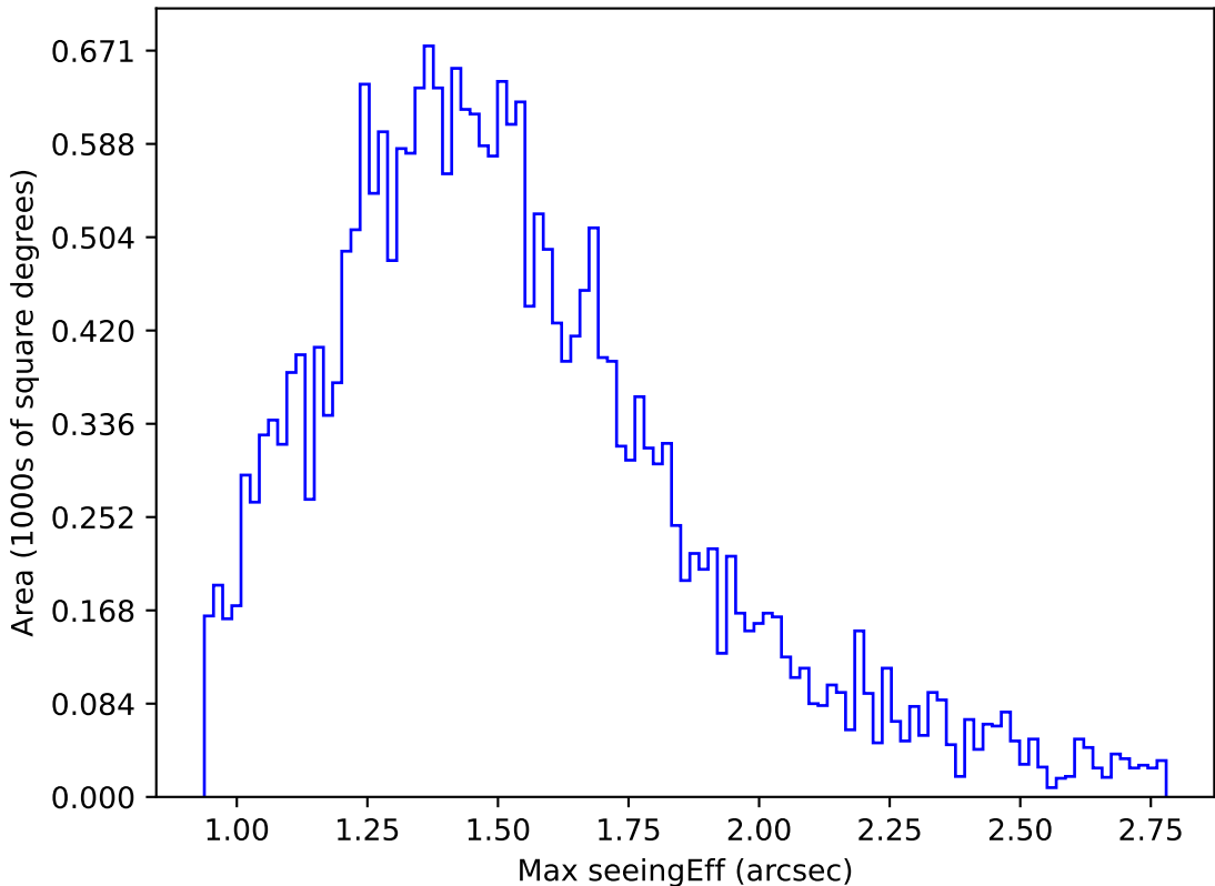
too_elab_r8_d3_ugrizy_v3.4_10yrs Yr 1 i band: Max seeingEff
