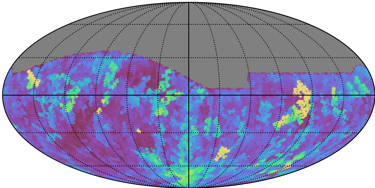
too_elab_r8_d3_ugrizy_v3.4_10yrs Yr 1 all bands: Max seeingEff
