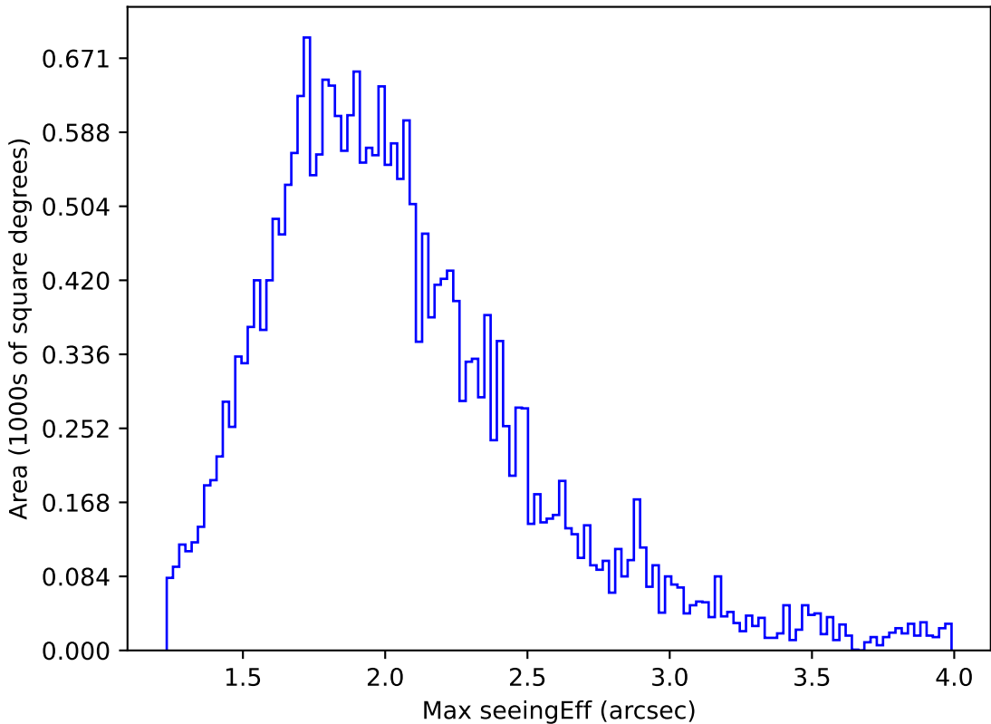
too_elab_r8_d3_ugrizy_v3.4_10yrs Yr 1 all bands: Max seeingEff
