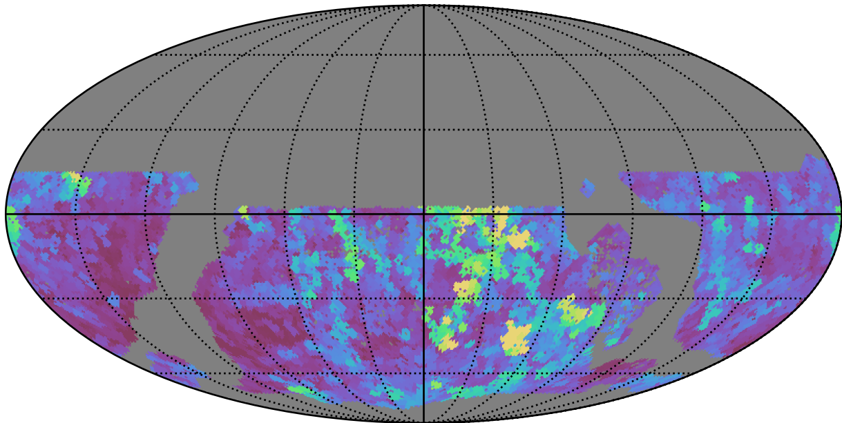
too_elab_r8_d3_ugrizy_v3.4_10yrs WFD z band: Max seeingEff
