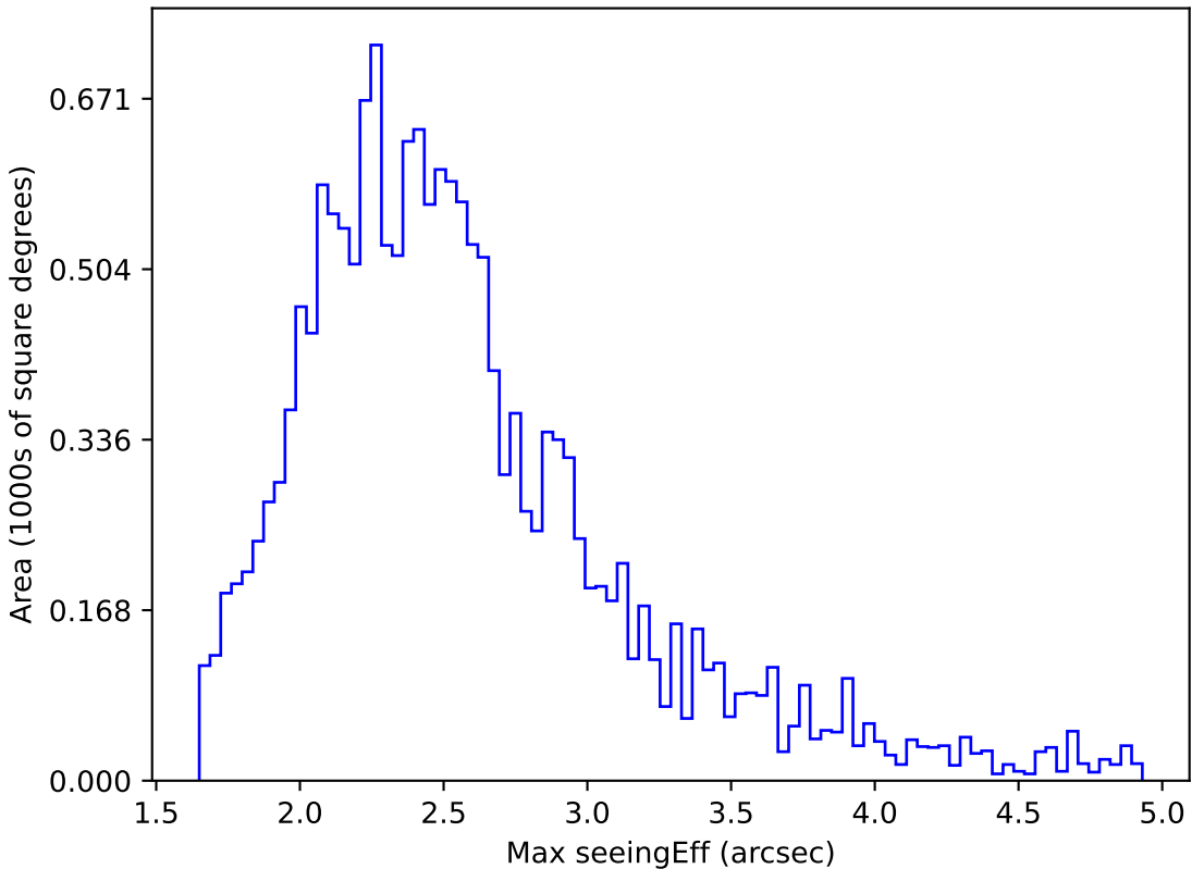
too_elab_r8_d3_ugrizy_v3.4_10yrs WFD z band: Max seeingEff
