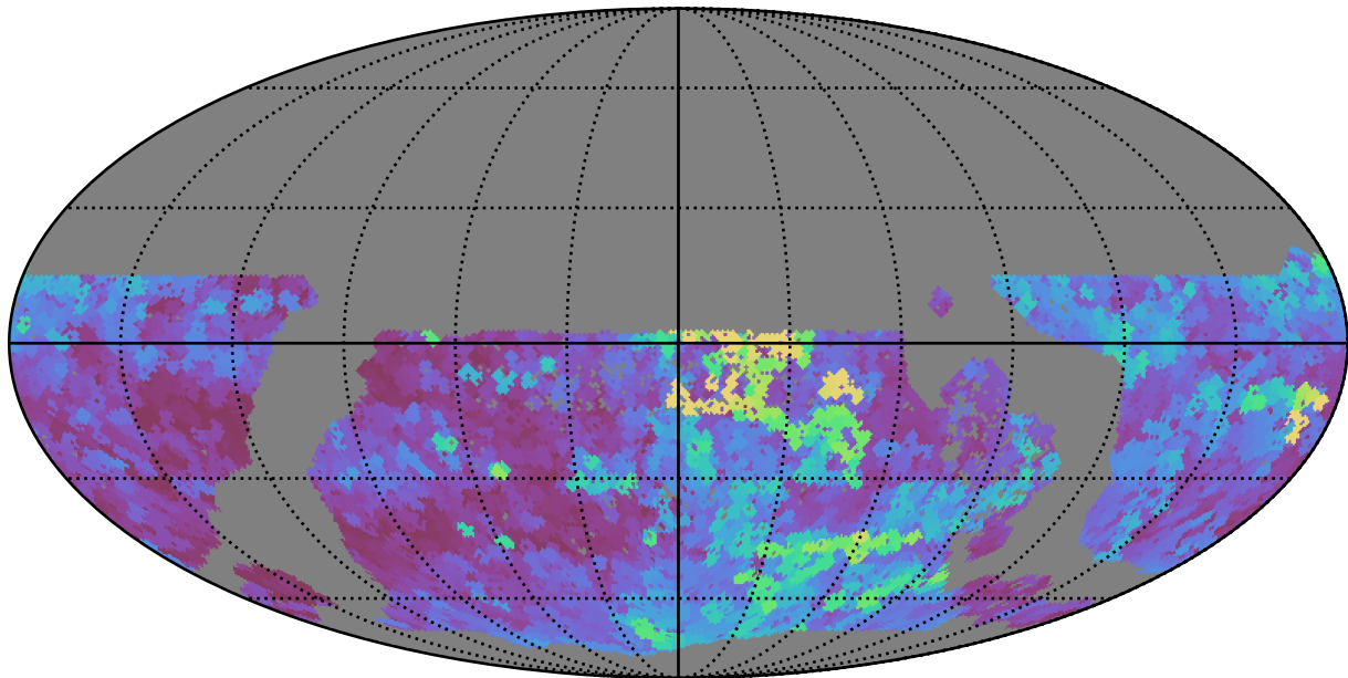
too_elab_r8_d3_ugrizy_v3.4_10yrs WFD y band: Max seeingEff
