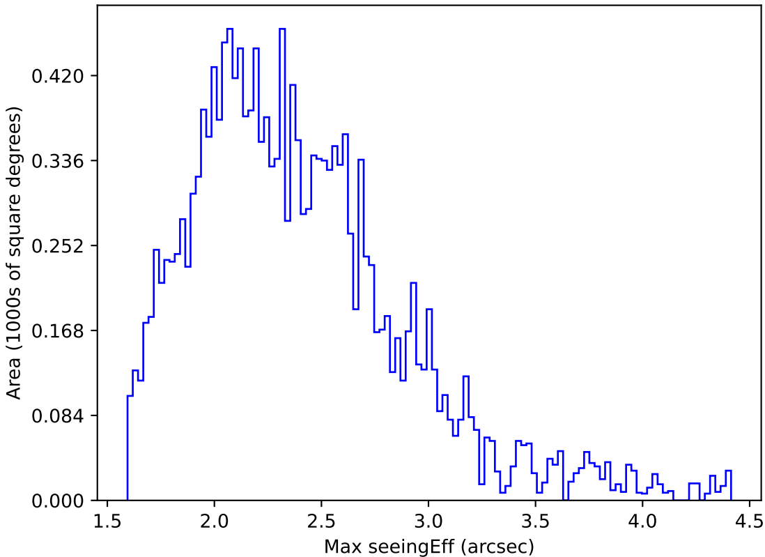
too_elab_r8_d3_ugrizy_v3.4_10yrs WFD y band: Max seeingEff
