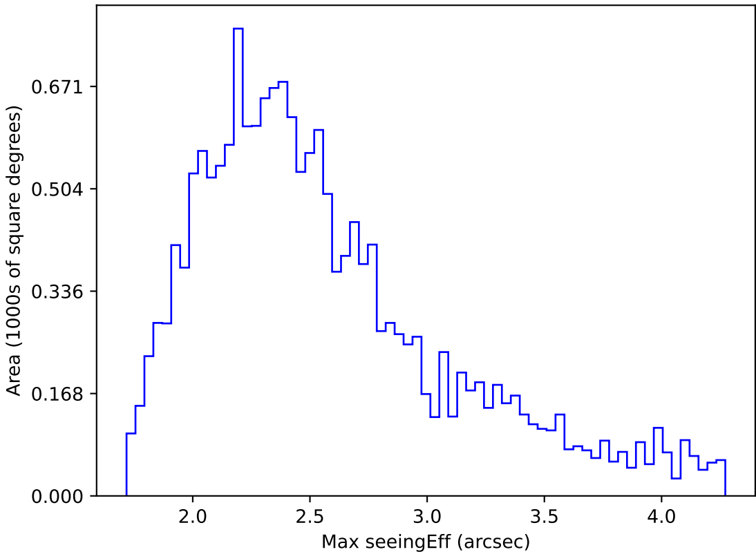
too_elab_r8_d3_ugrizy_v3.4_10yrs WFD u band: Max seeingEff
