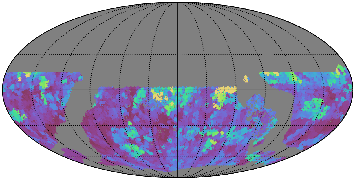
too_elab_r8_d3_ugrizy_v3.4_10yrs WFD r band: Max seeingEff
