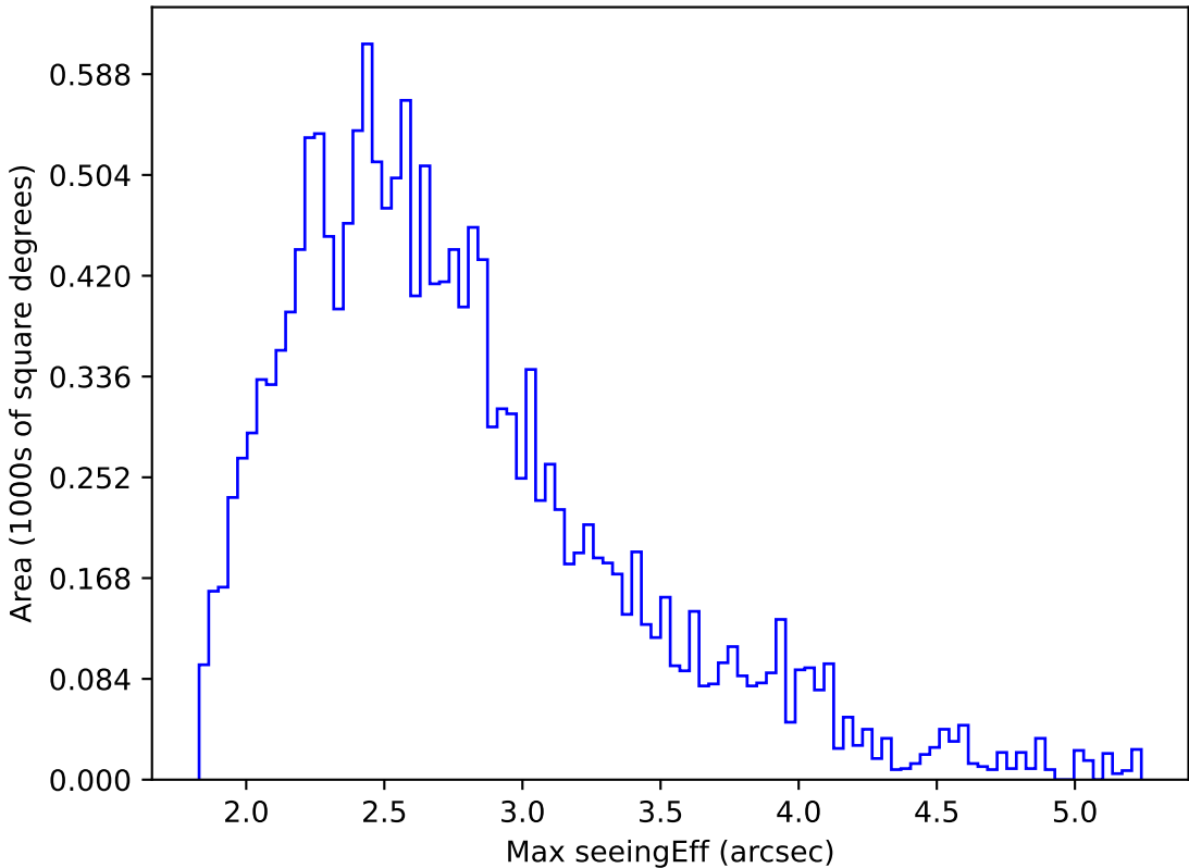
too_elab_r8_d3_ugrizy_v3.4_10yrs WFD r band: Max seeingEff
