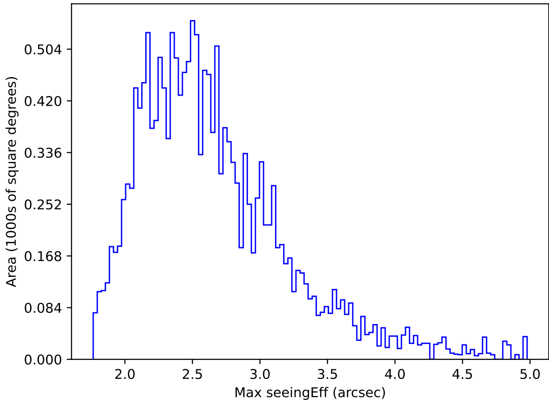
too_elab_r8_d3_ugrizy_v3.4_10yrs WFD i band: Max seeingEff
