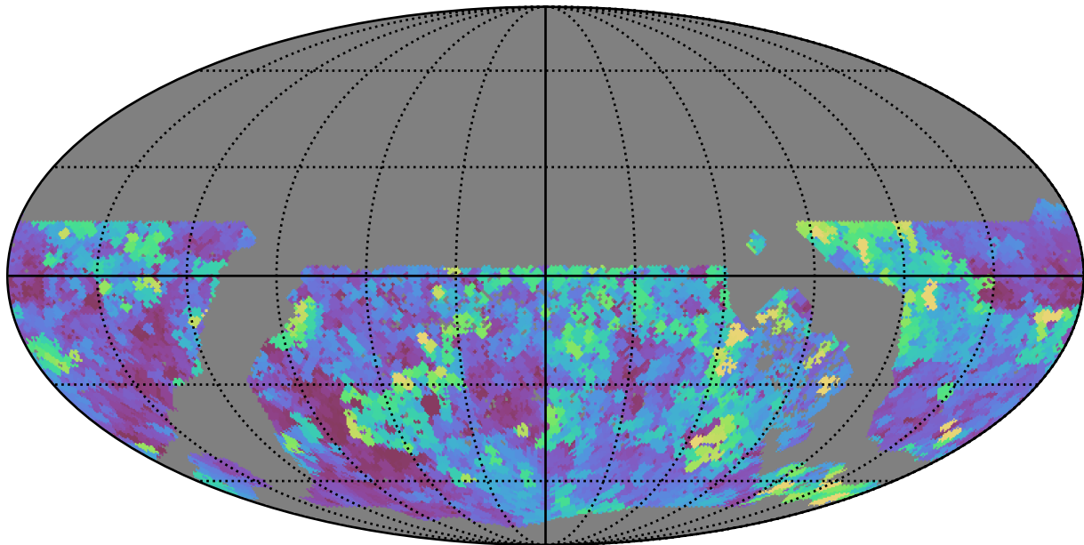
too_elab_r8_d3_ugrizy_v3.4_10yrs WFD g band: Max seeingEff
