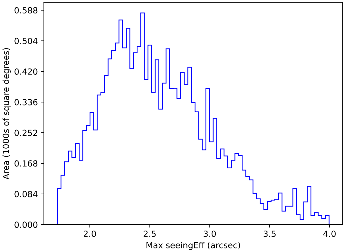
too_elab_r8_d3_ugrizy_v3.4_10yrs WFD g band: Max seeingEff
